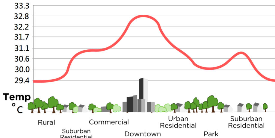
Diagram illustrating the heat-island effect in a US context. 8
